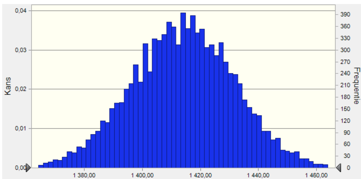
Figure 14: Histogram Monte Carlo simulation powerbanks
