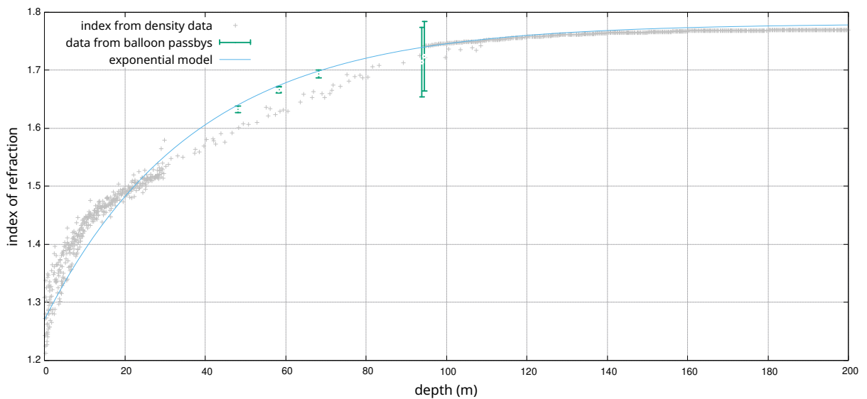
Figure B.1: Changing the linear index-density relation from n(z) = 1 + 0.78\rho(z)/\rho_0 to n(z) = 1 + 0.77\rho(z)/\rho_0 (shown here) doesn't impact the conclusion
