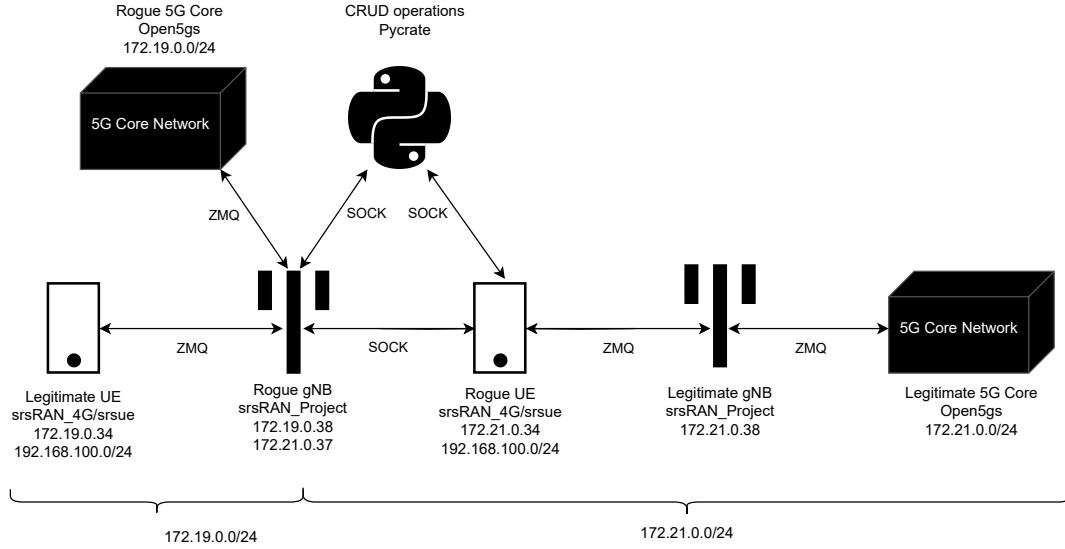
Figure 5.6: The ZMQ MITM setup architecture.
