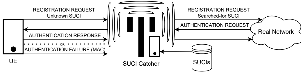
Figure 4.27: The probing step of the attack phase of the SUCI-catcher as described in [Chl+21].
