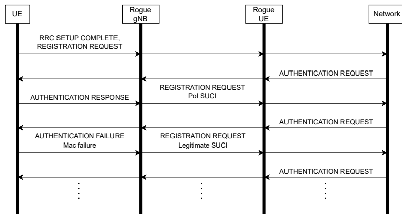
Figure 5.13: The observed signaling of a test of the SUCI catcher attack using the setup shown in Figure 5.6.
