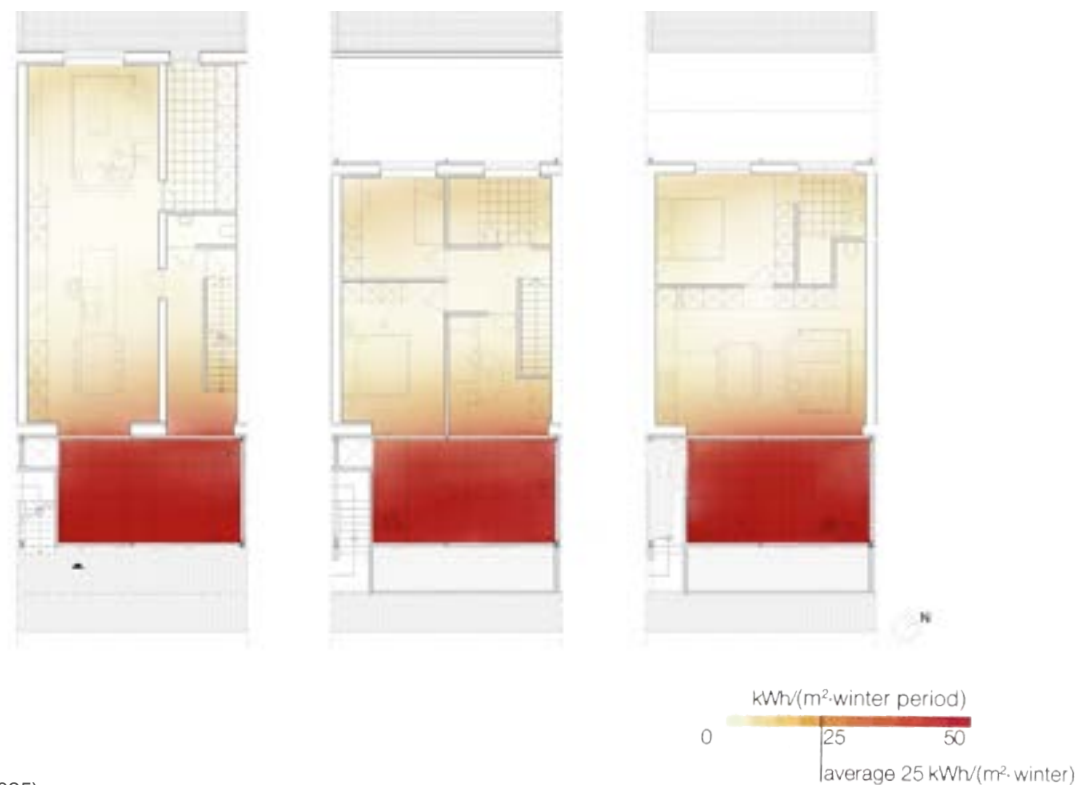
Figuur 4.61 Solar heat gains in winter
