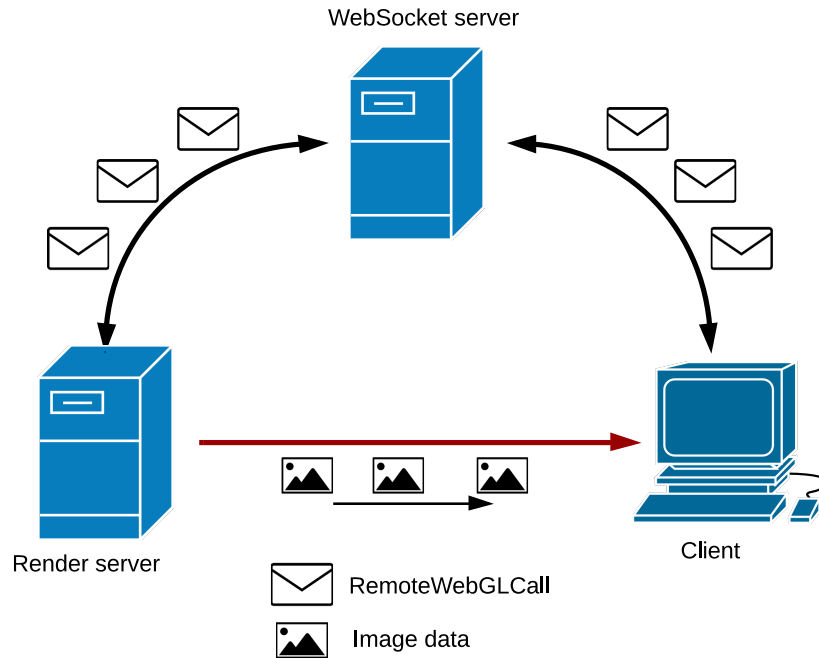
Figure 6.3: Message exchange in the Remote WebGL Rendering solution. The client sends RemoteWebGLCalls to the server. The server responds with new frames, transported as BASE64 encoded images.
