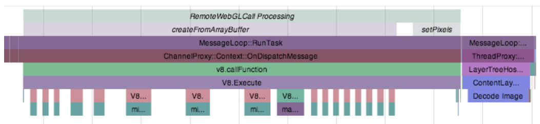
Figure 6.7: Processing of one RemoteWebGLCall with image data (client). The topmost bar shows covers the full processing of a RemoteWebGLCall. The createFromArrayBuffer bar shows that most time is spend deserializing the frame. The binary-to-text conversion appears to be very slow. It also shows a lot of garbage collector pauses.
