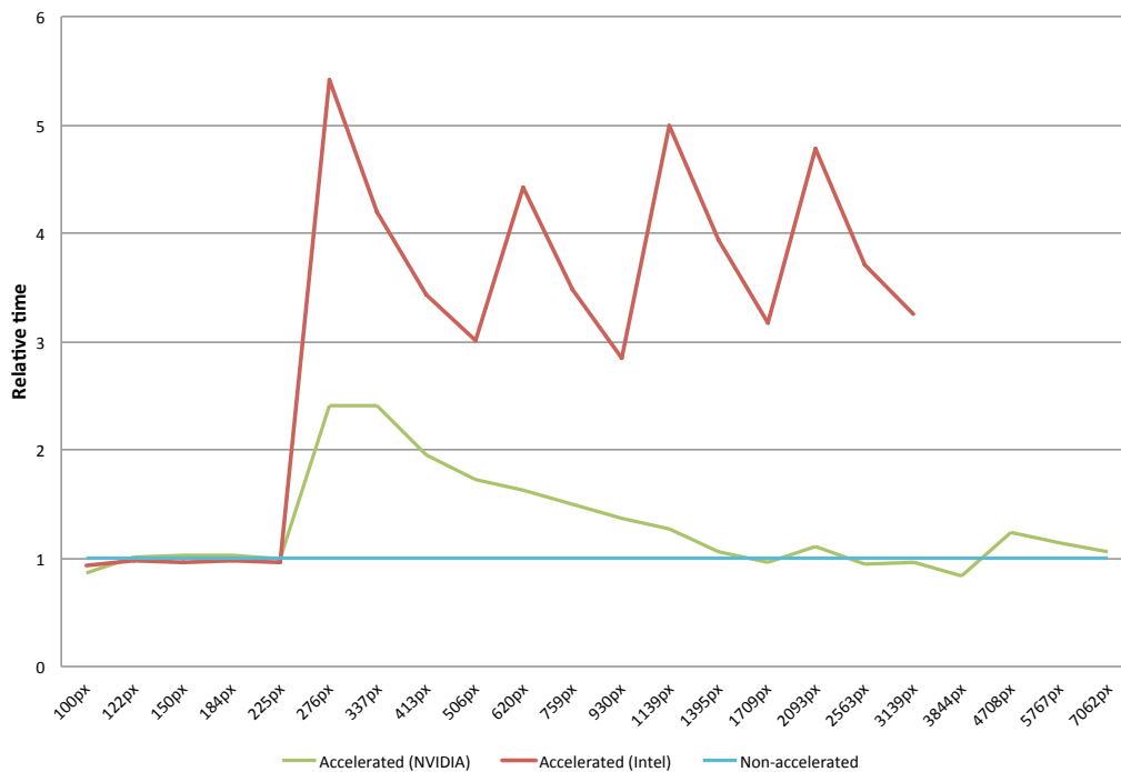
Figure 4.10: Relative performance comparison of getImageData calls on canvasses of different size. The performance drop is clearly visible here when the canvas becomes hardware accelerated.
