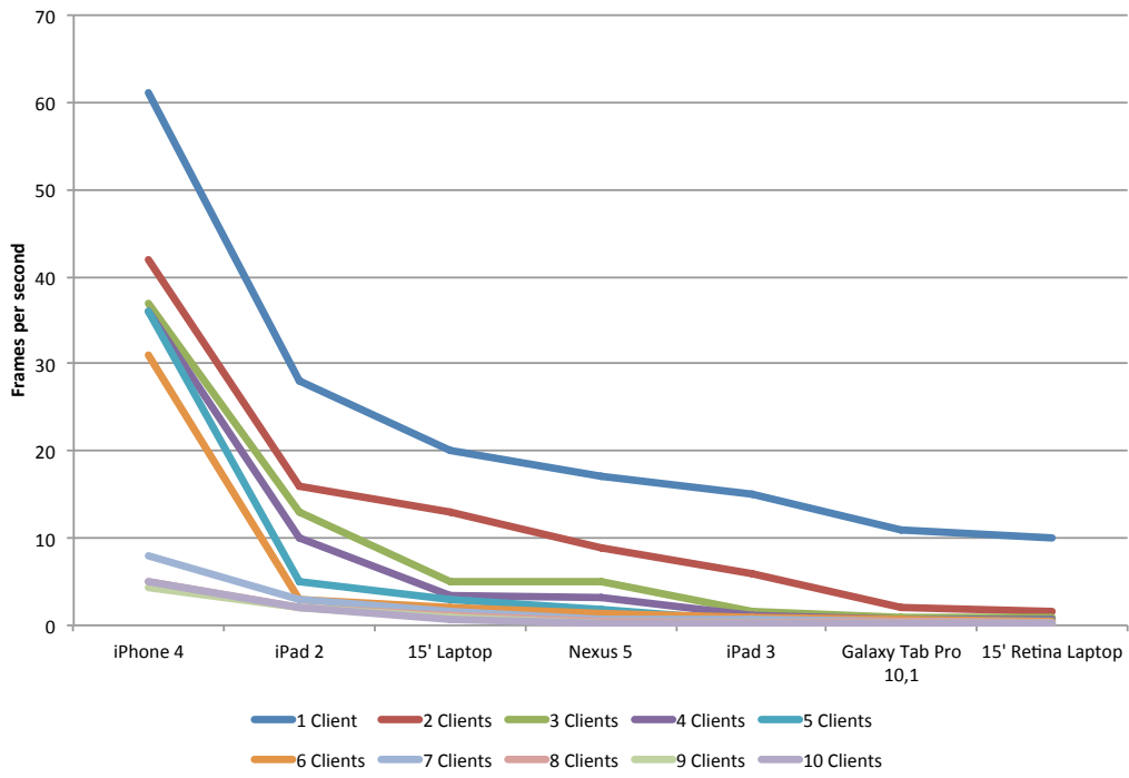
Figure 6.11: Results of the server scalability tests for the original (image based) version.
