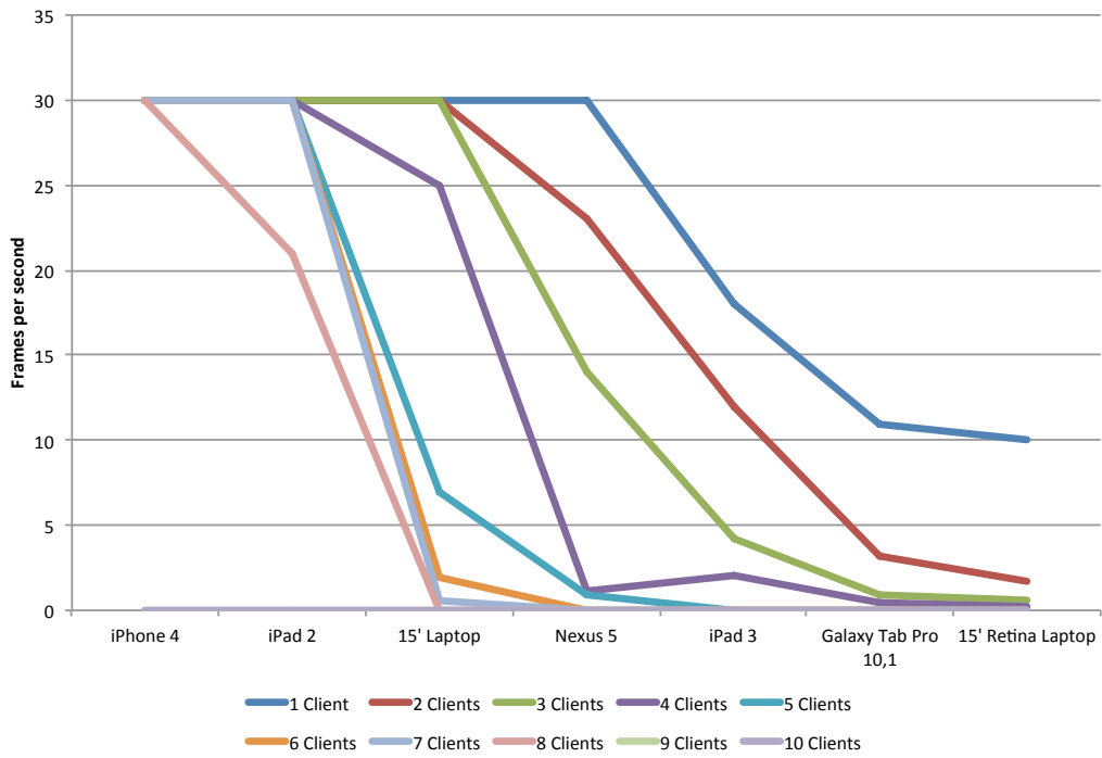
Figure 6.12: Results of the server scalability tests for the WebRTC based version. The video stream has a maximum frame-rate of 30fps.
