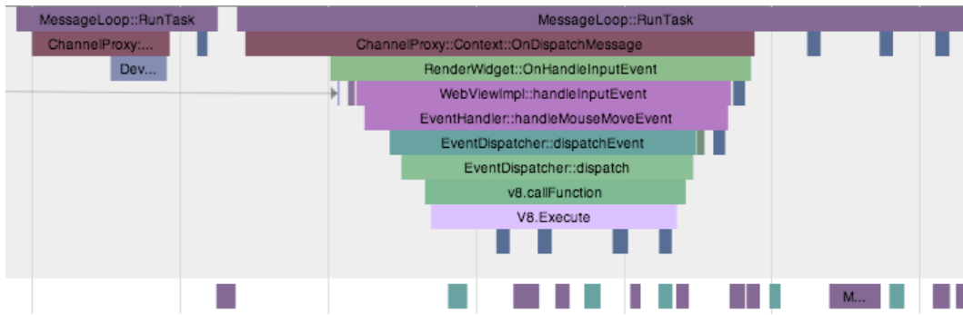
Figure 4.5: Screenshot of the Trace Event Profiling Tool
