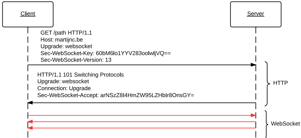
Figure 2.1: The WebSocket handshake starts with the HTTP protocol and is upgraded once the handshake is complete.
