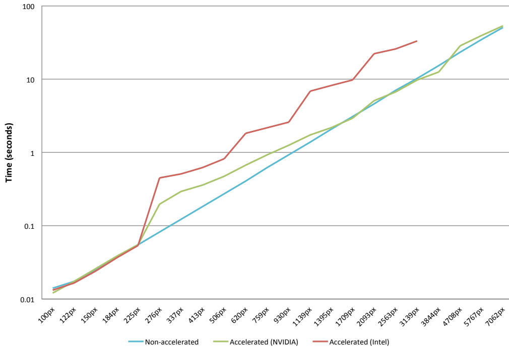
Figure 4.9: Performance comparison of getImageData calls on canvasses of different size. The performance drop is clearly visible here when the canvas becomes hardware accelerated.
