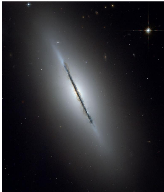
Figuur 2: NGC 5866. (Hubble Space Telescope)
