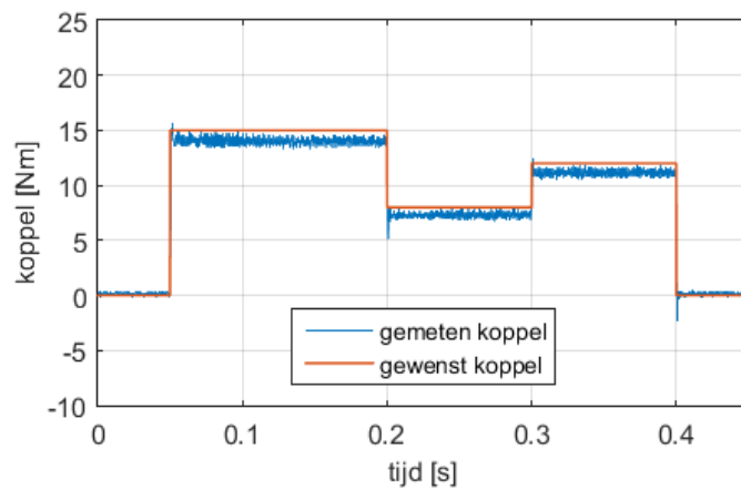
Figuur 3: Deadbeat controller
